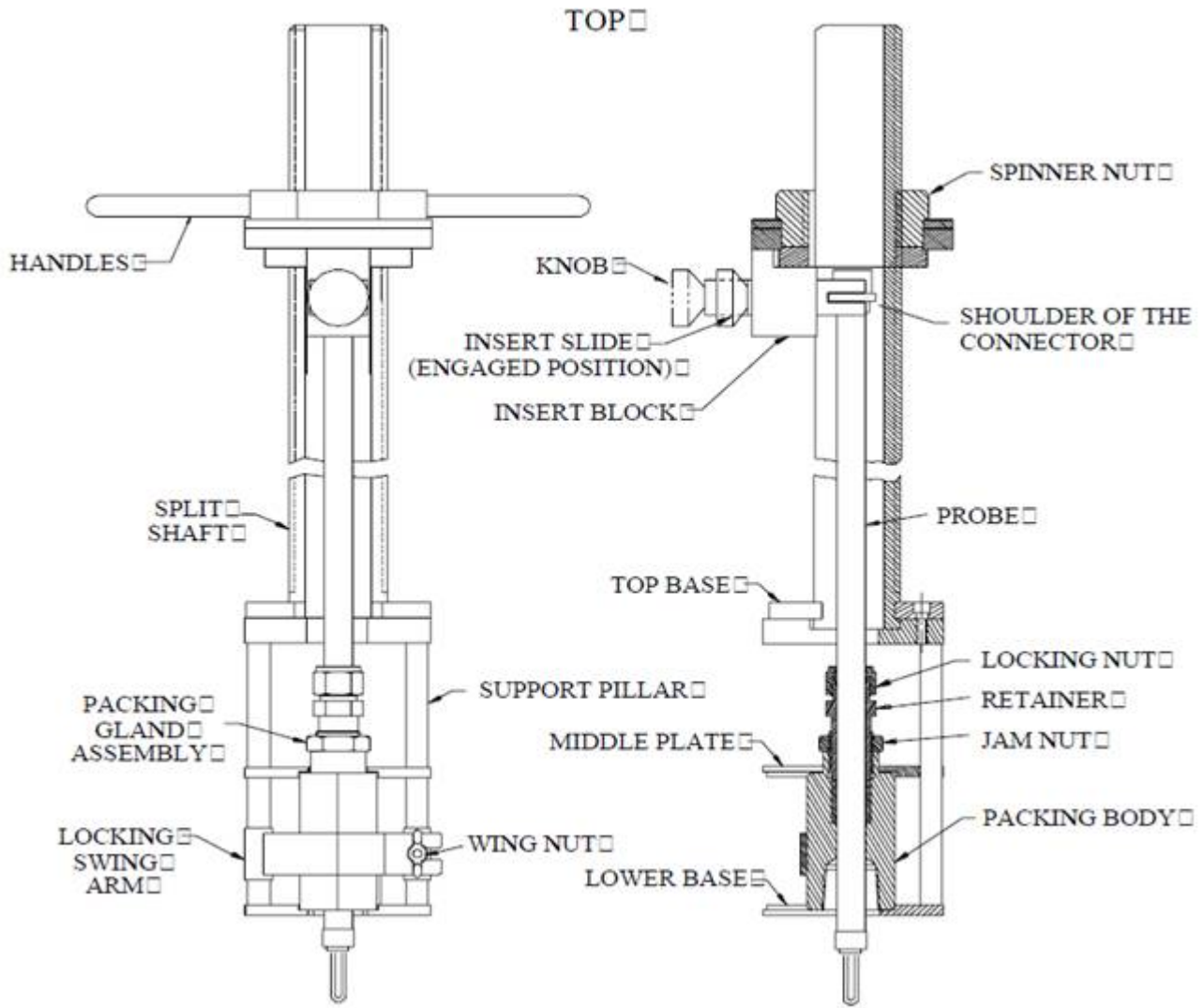
Figure 1. Easy Tool Retracting System
