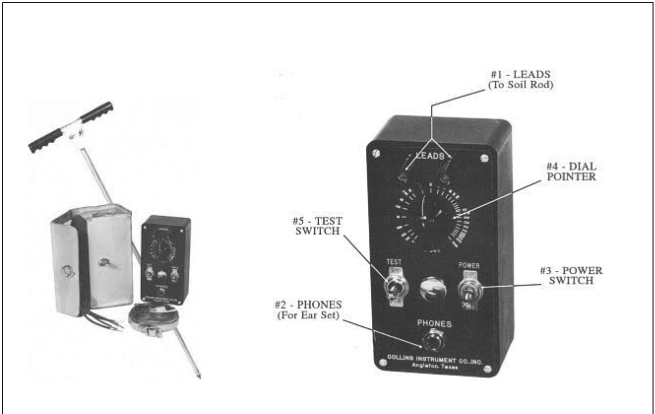
Collins Single probe meter
