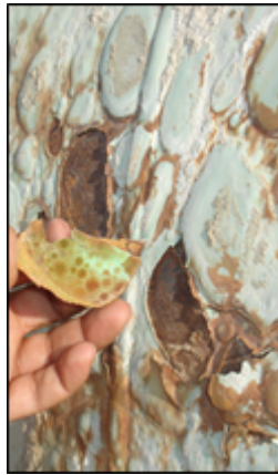
Figure 1: Bubbled or Blistered coating
