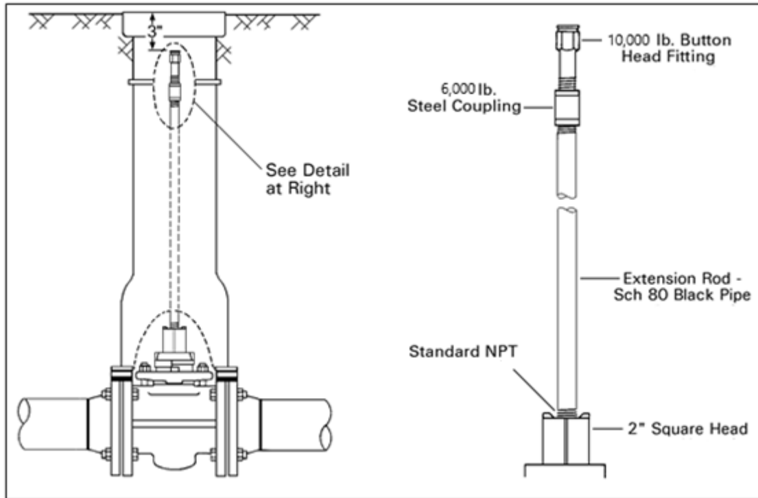
Figure A2 - Typical Plug Valve Lubrication Extension Installation
