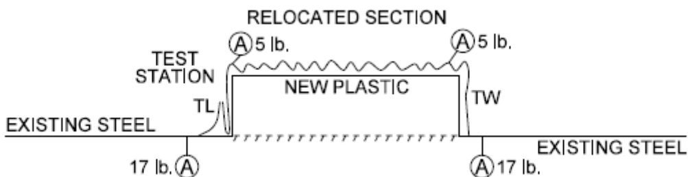
Figure 11. Relocating Existing Steel with Plastic
