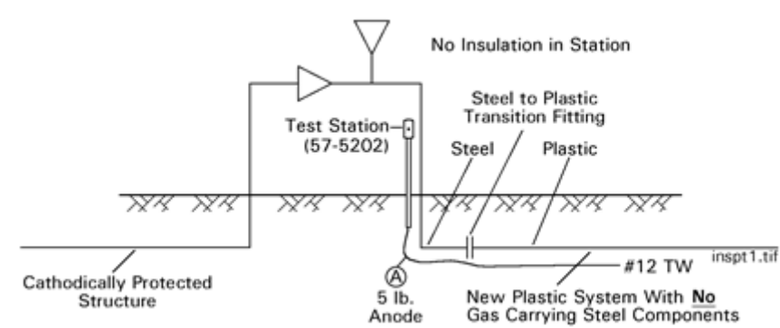
Figure 2. Distribution Station - New Plastic Outlet System
