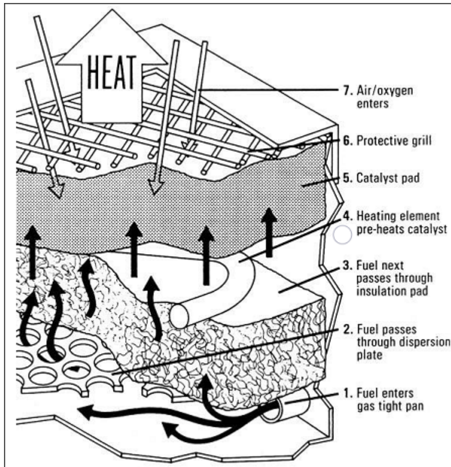
Figure 4: Catalytic Heater Diagram
