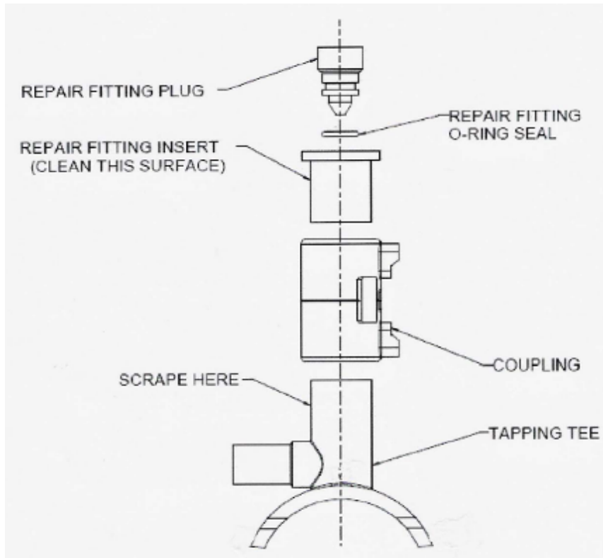
Figure 1: Repair Kit Assembly
