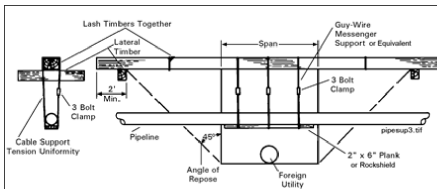
Figure 3: Type "C" Support
