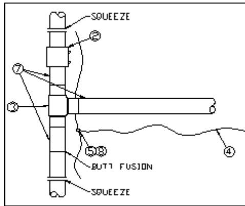
Figure 2 In-line Tee
