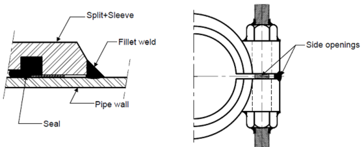
Figure 2: Seal Welding the Split+Sleeve
