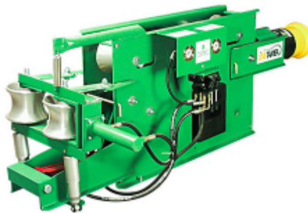
Figure 3. LineTamer
