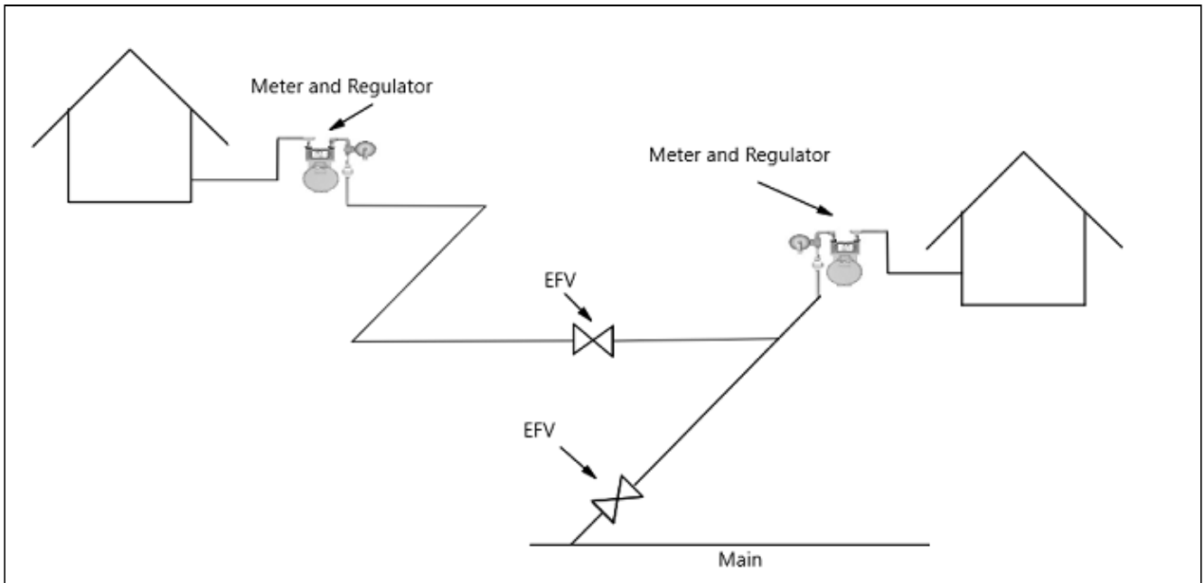
A-4. EFV installation on a new branch service line off an existing primary service line.
