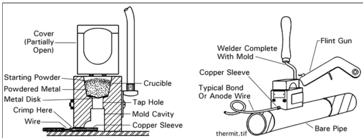
Typical Thermite Weld Configuration
