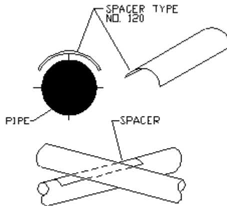
Figure 5 Spacer Installation
