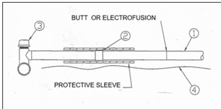
Figure 5 Mueller Tee and Steel transition fitting to PE Pipe
