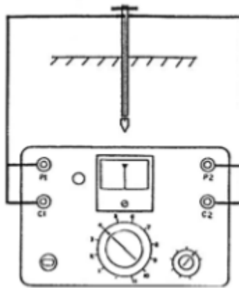
Figure 2 Single Pin Method Schematic
