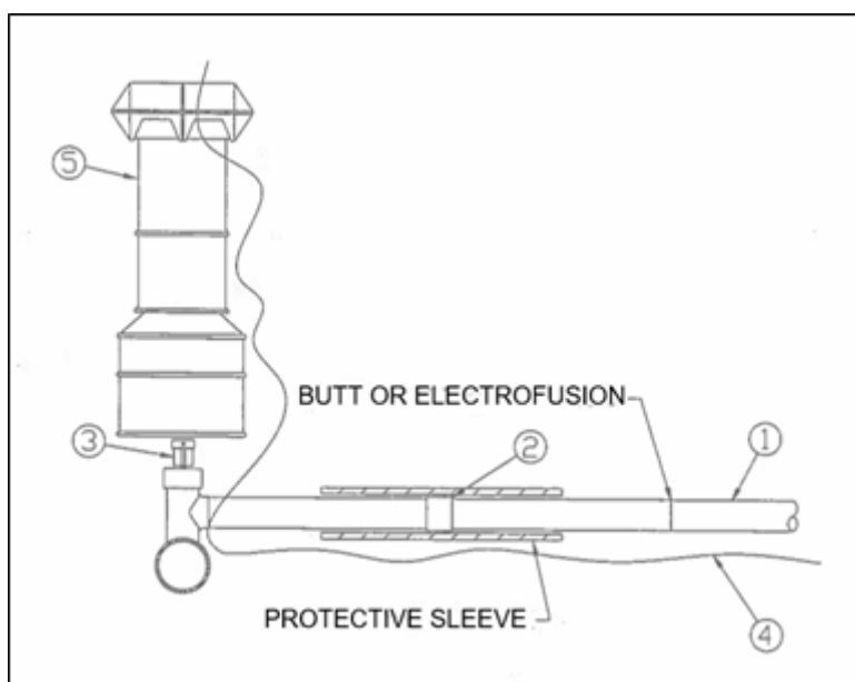
Figure 6 Mueller Curb Valve Tee and Steel Transition fitting to PE Pipe
