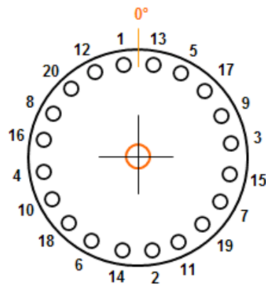
20 Bolts Sequential Order
