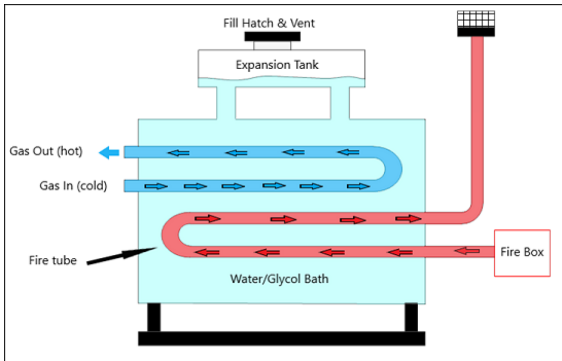
Figure 2: Indirect Water Bath Heater
