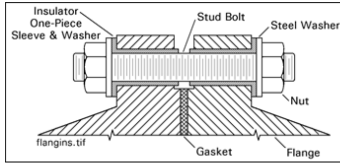
Figure 13. Double-bolt Insulators
