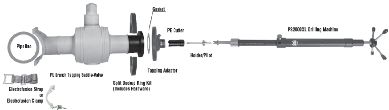
Figure 1: Tapping Setup View
