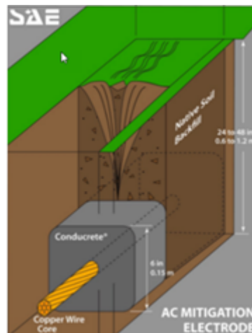
Figure 7 Copper Cables Used for AC mitigation
