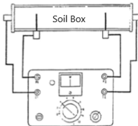
Figure 3 Soil Box Resistivity Measurements
