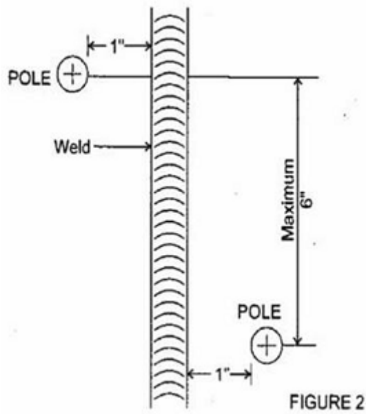
Figure 2: Magnetic Particle Inspection Sequence
