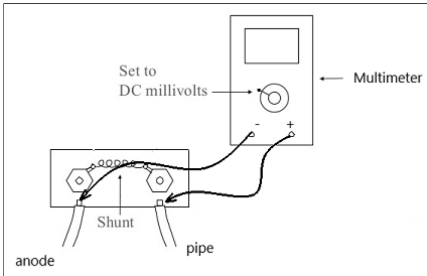
Figure 5 Multimeter in circuit Method
