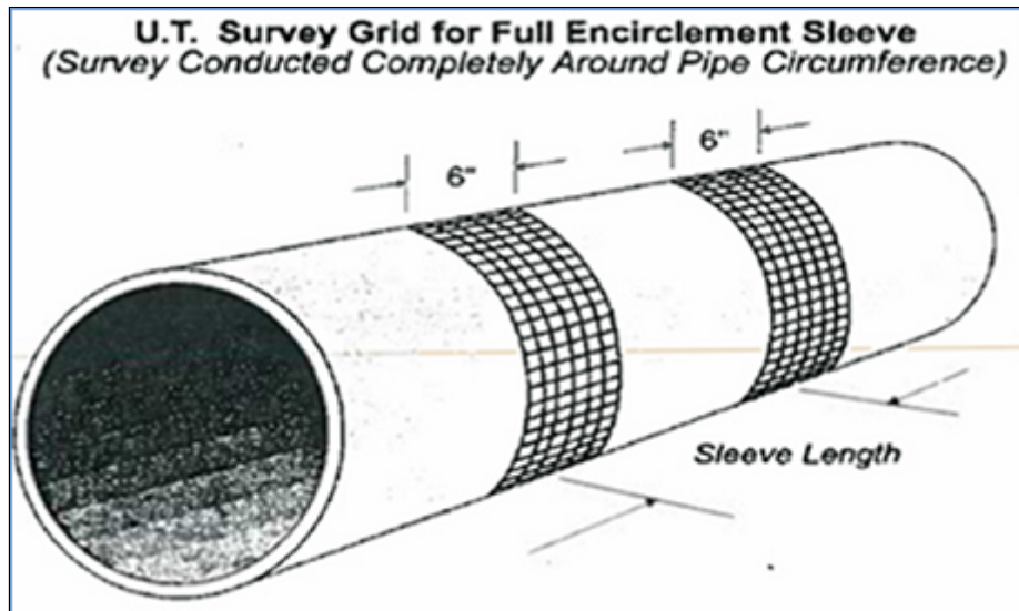
Figure 1: UT Survey - Full Encirclement
