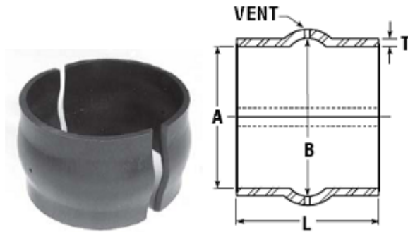
Figure 1: Dresser Style 110 Sleeve
