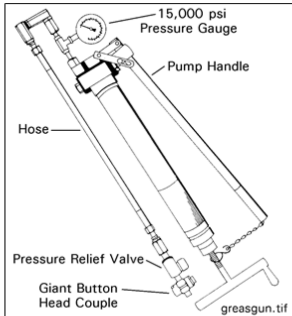
Figure A1 - Typical Plug Valve Lubrication Channels and Typical Grease Gun
