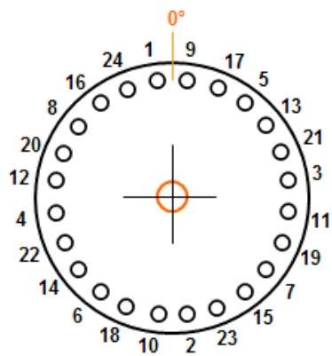
24 Bolts Sequential Order
