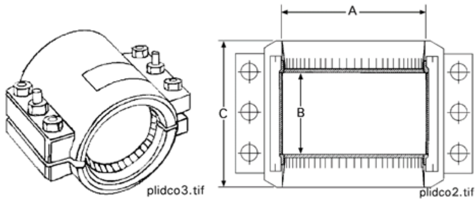
A-2. Plidco Split+Sleeve - Basic Unit
