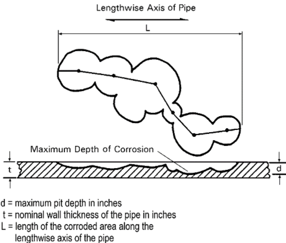
Figure 1 Pit Measurement Criteria
