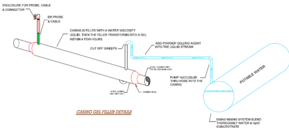
Figure 6: Typical Casing Gel Filler Details
