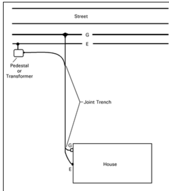
Figure 3 Trench Route
