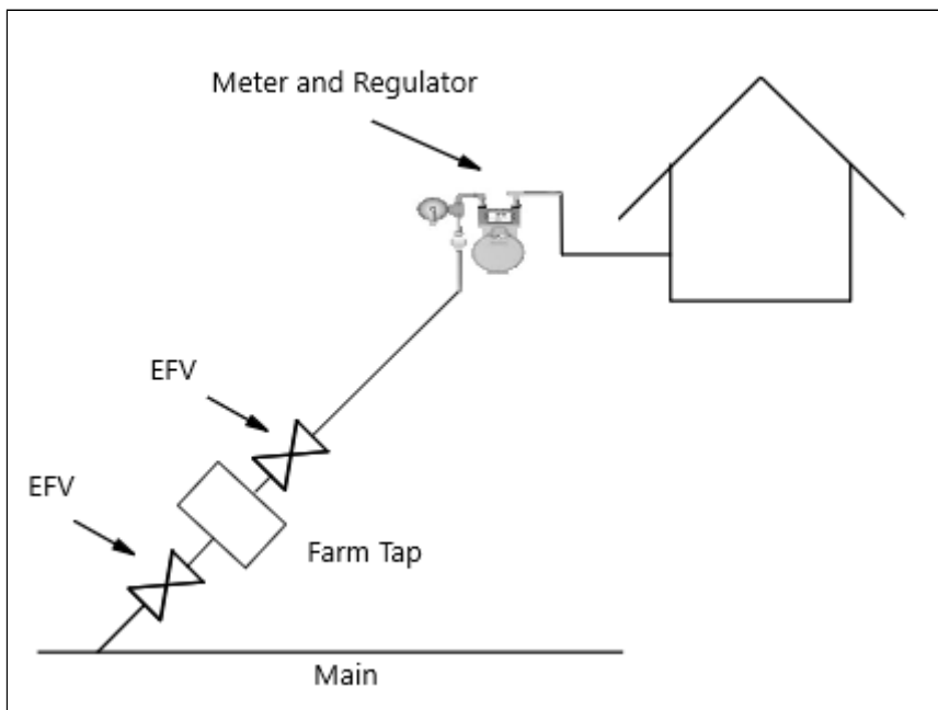
A-5. EFV installation on farm tap
