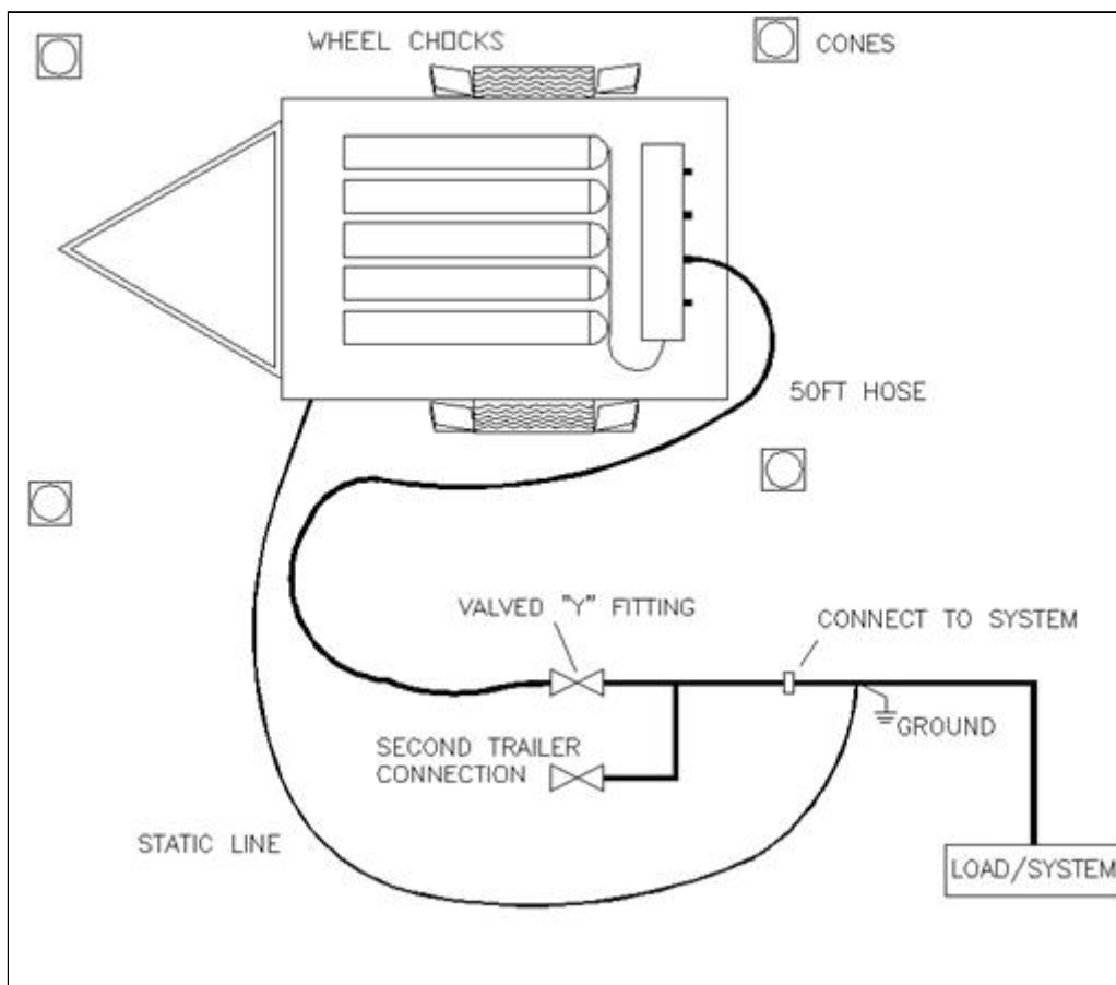
Figure 4: Typical CNG Trailer Application
