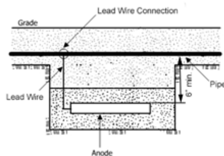
Figure 2. Typical Horizontal Installation
