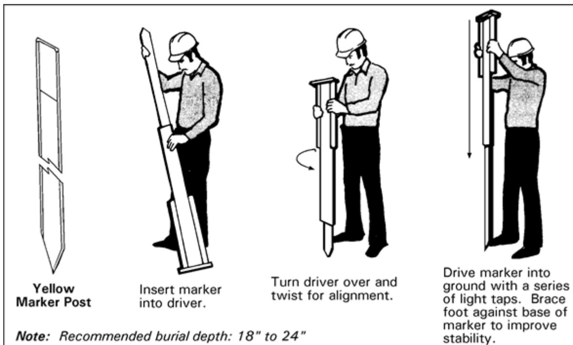
Figure 5: Pipeline Marker Post Driver Installation
