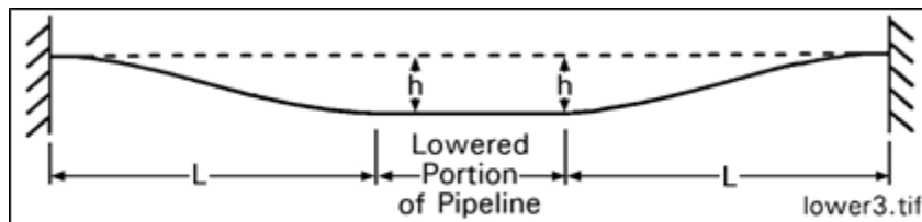
Figure 1 Steel Pipe Lowering Schematic
