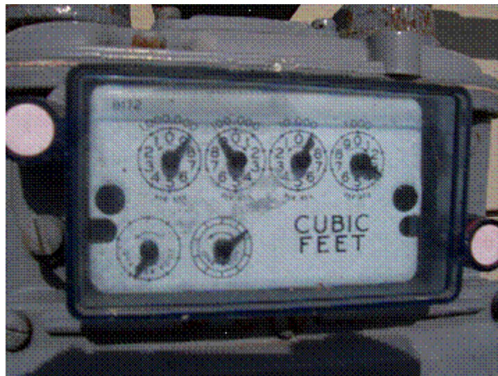
Figure 1: Gas Meter Index (Test hands at lower left)
