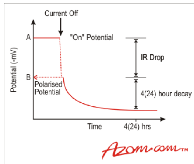
Figure1. Potential Decay Curve
