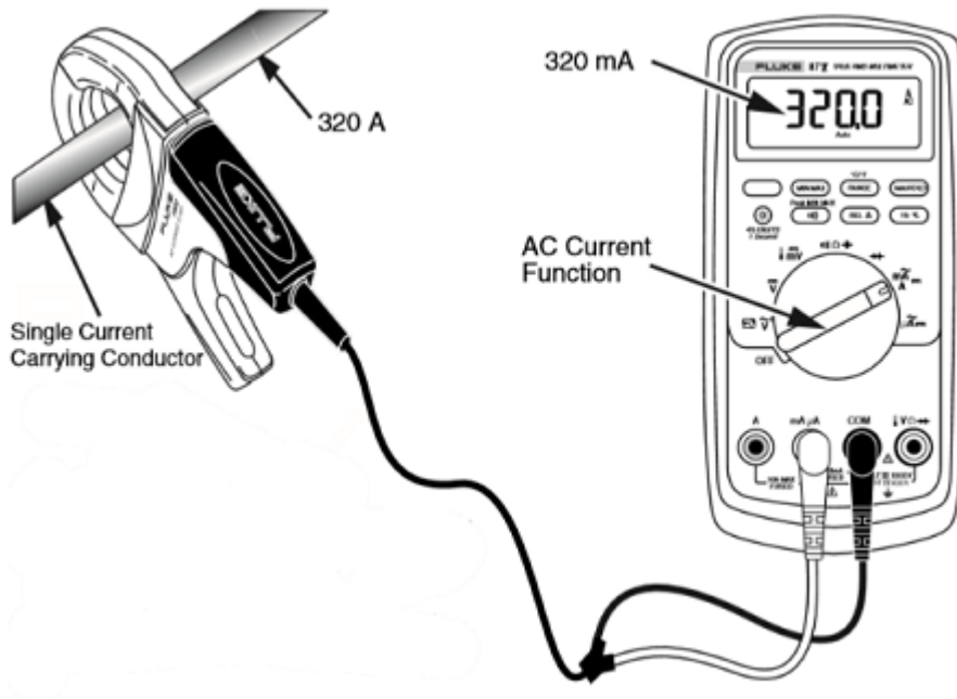
Figure 3 Typical non-contact ammeter.
