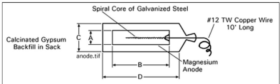
Figure 3 AIC Approved Anode
