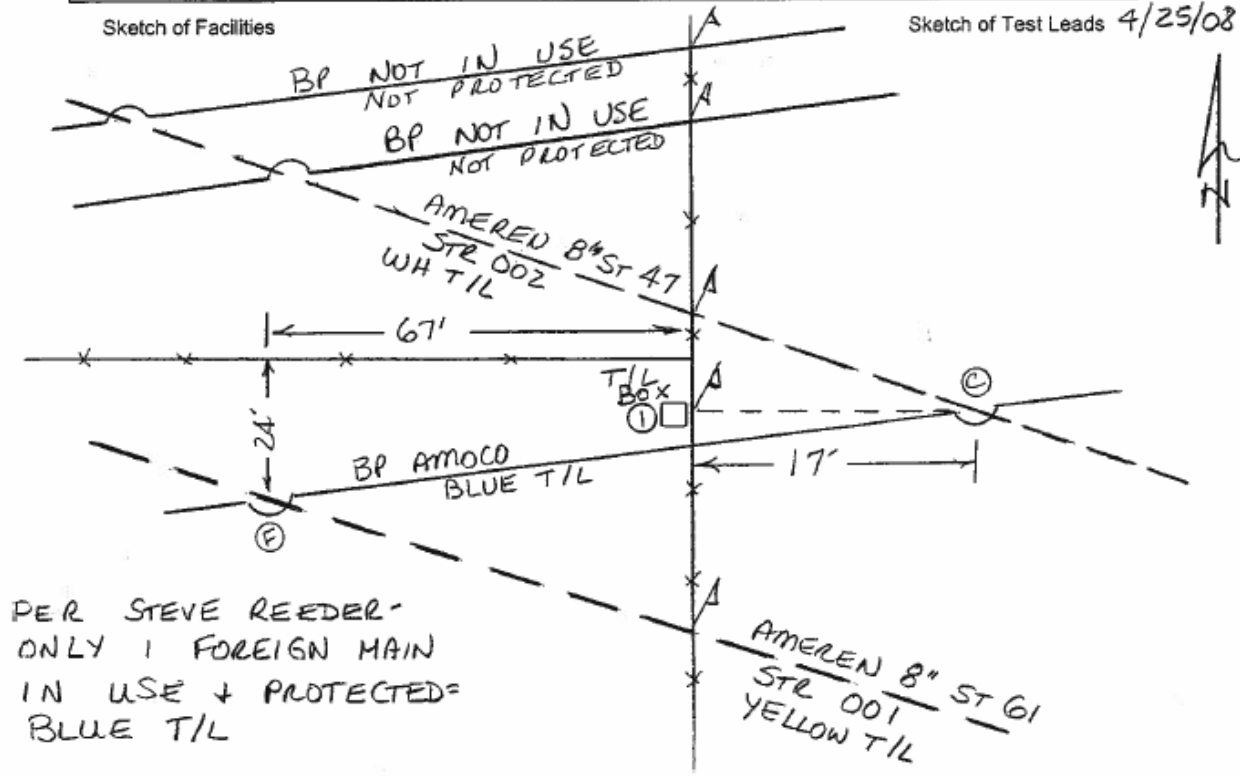
Figure 2 Pipeline Crossing
