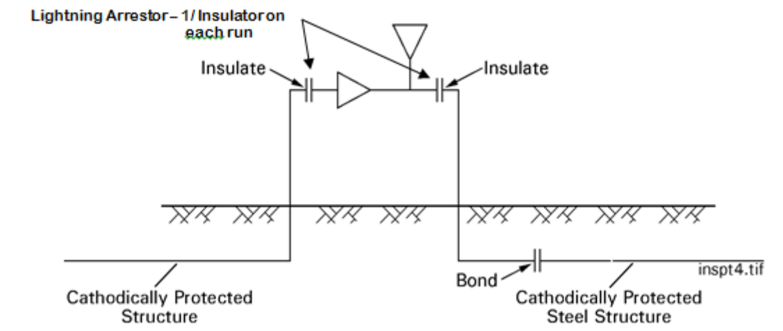
Figure 4. Delivery Station
