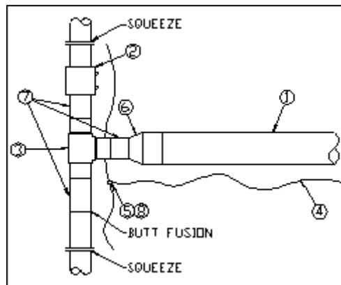
Figure 3 In-line Tee with reducer
