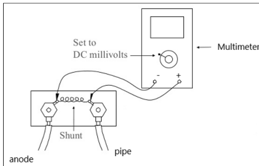
Figure 4 Shunt and Multimeter Methods
