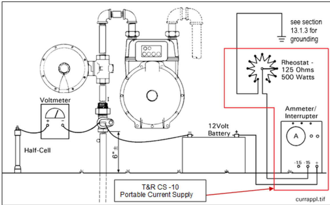
Figure 7 Schematic of Typical Current Application (See specific instructions for T&R CS 10 connections)
