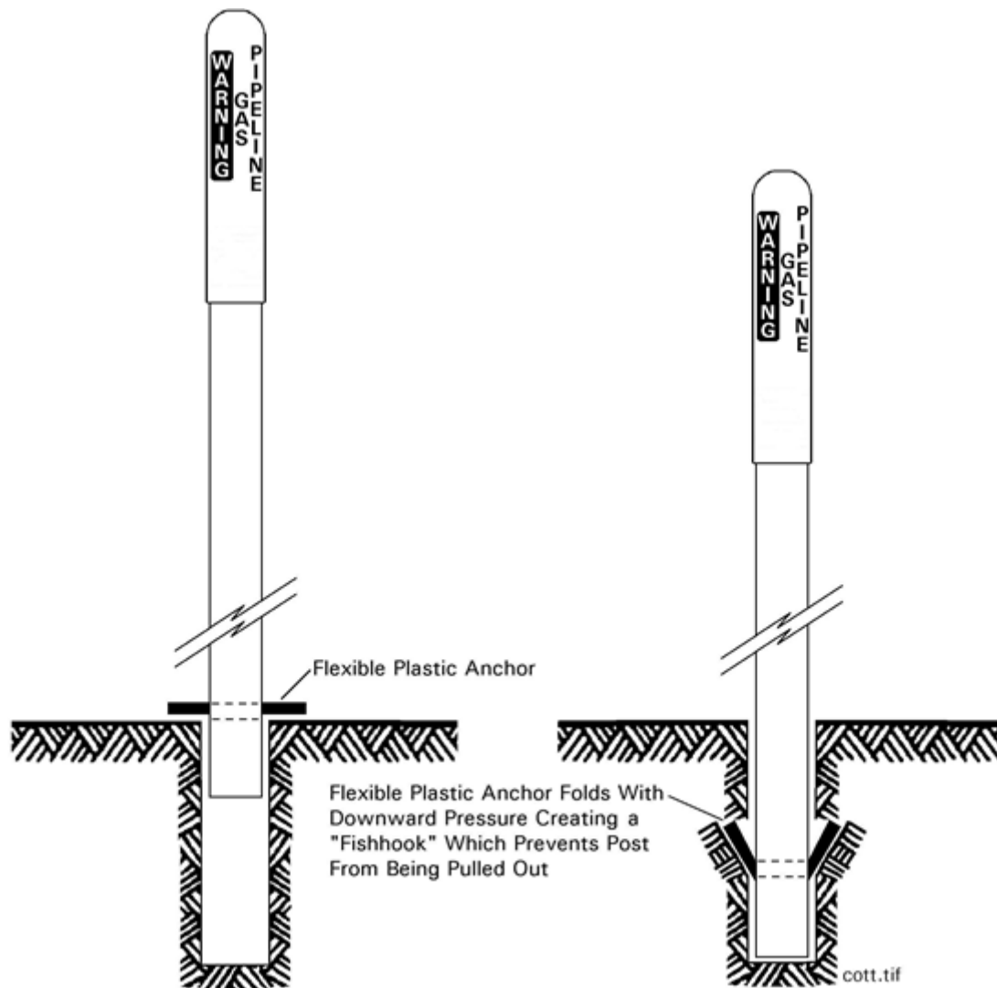
Figure 2: COTT Pipeline Marker Installation (Typical)
