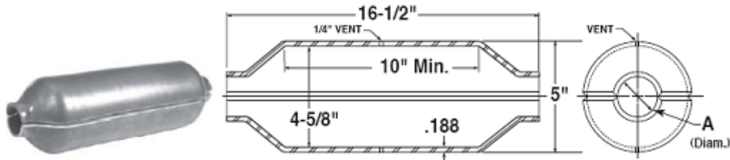
Figure 3: Dresser Style 220S Sleeve
