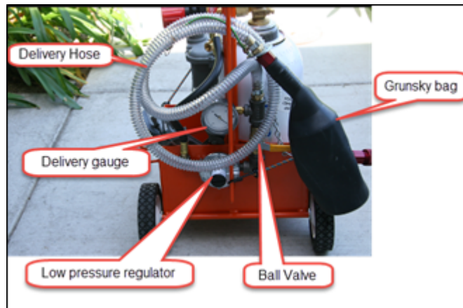
Figure 1: Grunsky Apparatus
