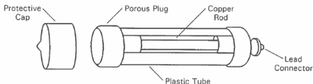
Figure 2. Copper Sulfate Reference Cell
