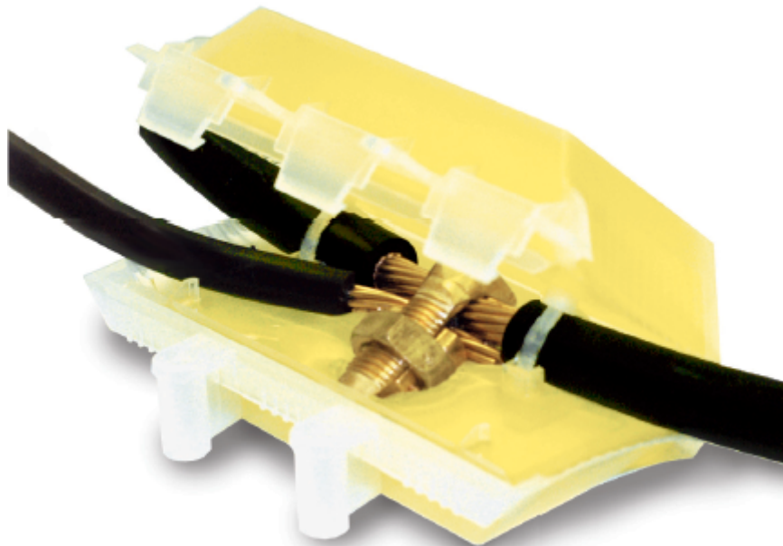
Dryconn VisiLock with Smart Gel Anode Splice Box
