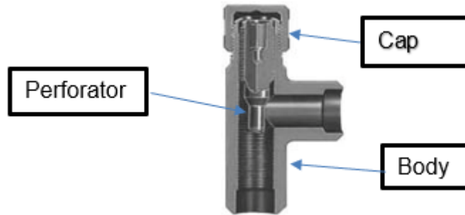
Figure 1: AUTOPERF Tee and AUTOPERF Transition Tee
