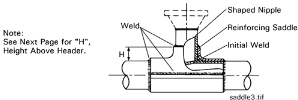
Figure 2: Full Encirclement Reinforcing Saddle - Typical Installation
