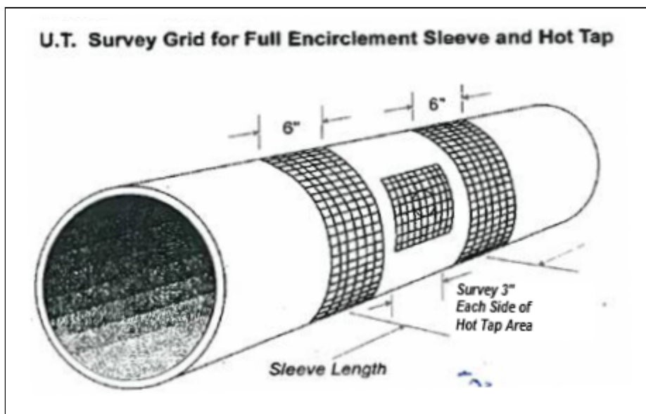
Figure 2: UT Survey - Full Encirclement with Hot Tap
