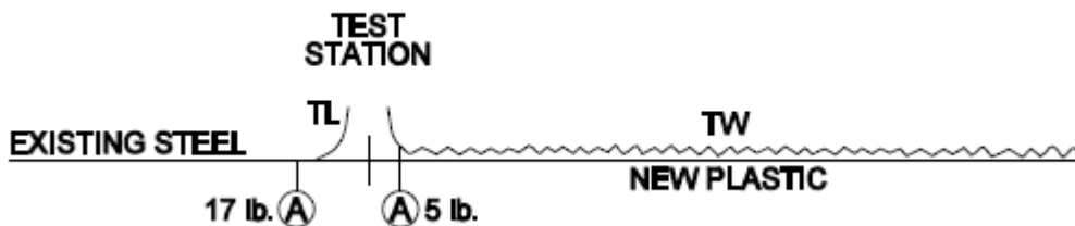
Figure 9. Extending New Plastic from End of Existing Steel.
