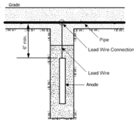
Figure 1. Typical Vertical Installation
