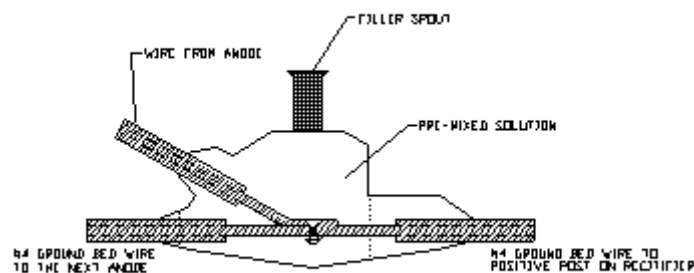
Anode Splice Box 3M A Scotchcast Resin Kit (90-B1)
