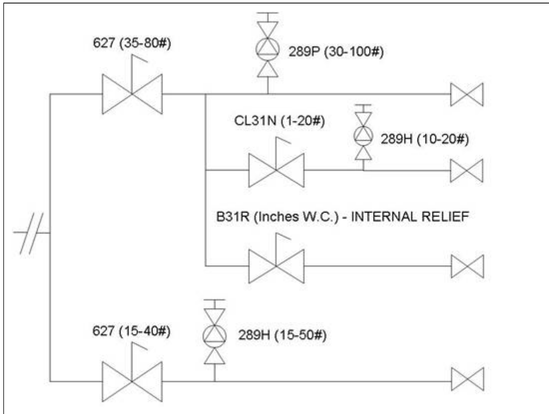
Figure 2: Typical Regulator Connections on CNG Trailers
