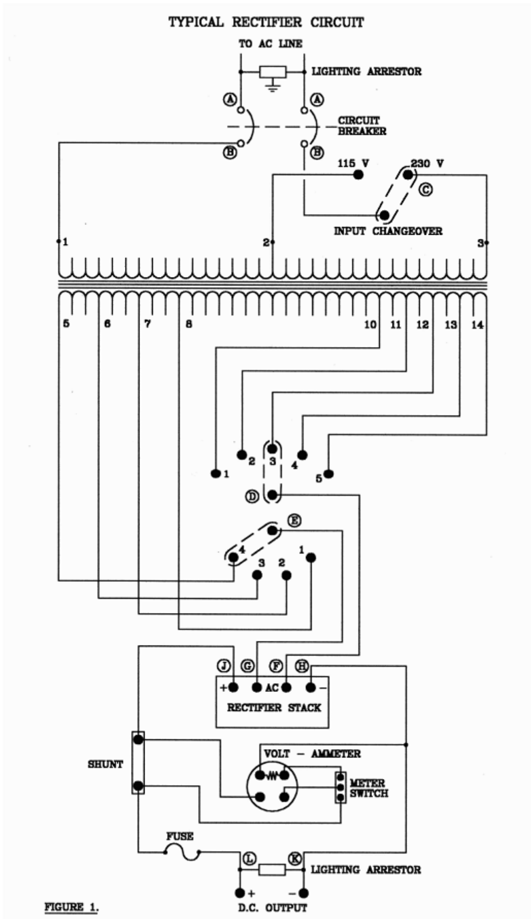
Figure 1 Typical Rectifier Circuit
