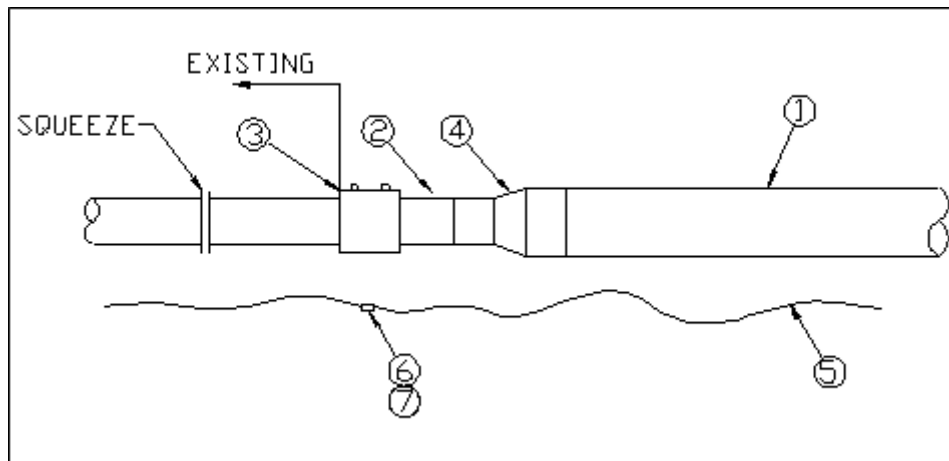
Figure 2 Main Extension, PE Pipe, Increasing size
