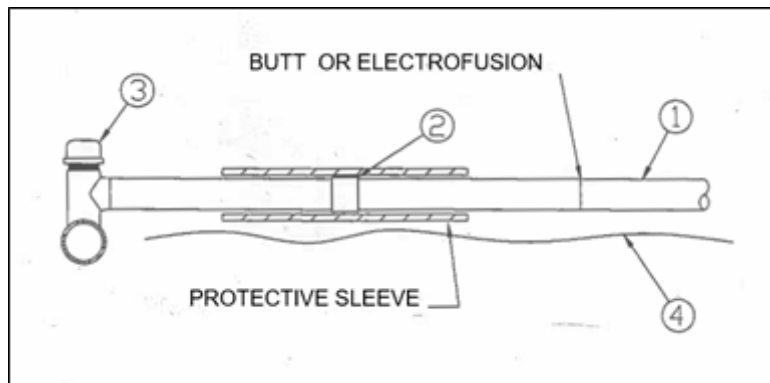
Figure 8 TDW Tee with Steel Transition fitting to PE Pipe
