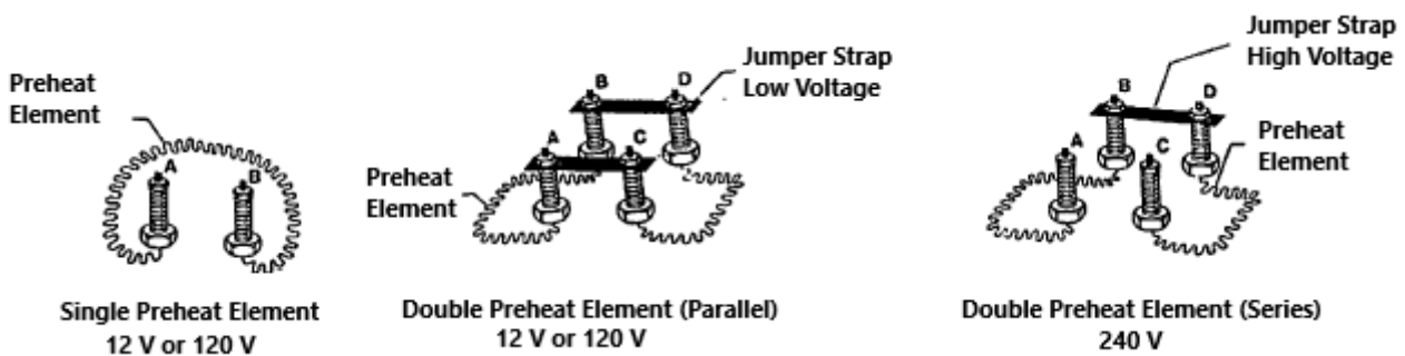
Figure 6: Catalytic Heater Preheat Terminals
