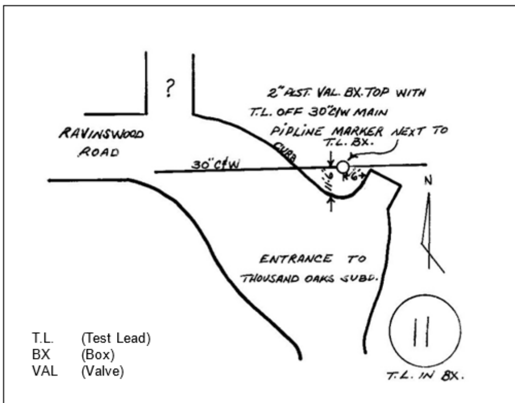
Figure 1 Test Point Detail Sketch
