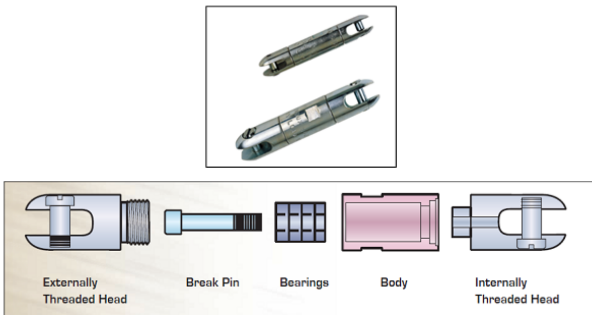
Figure 2: Condux Swivel (Information available online here .)
