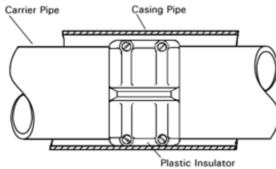
Figure 3: Insulator
