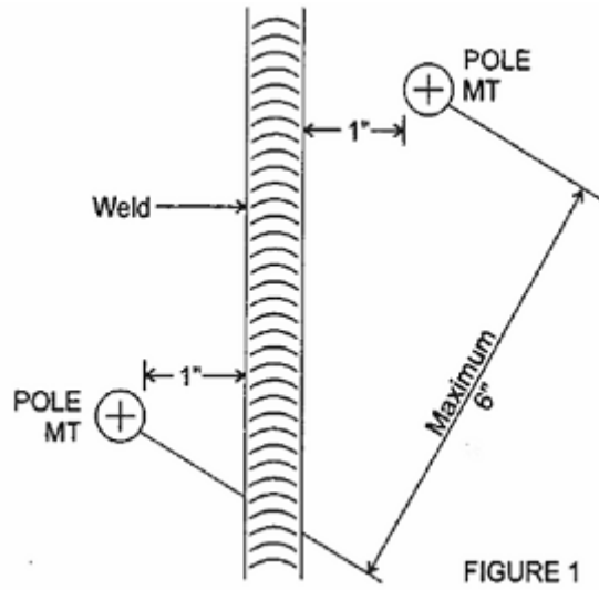
Figure 1: Magnetic Particle Inspection Sequence
