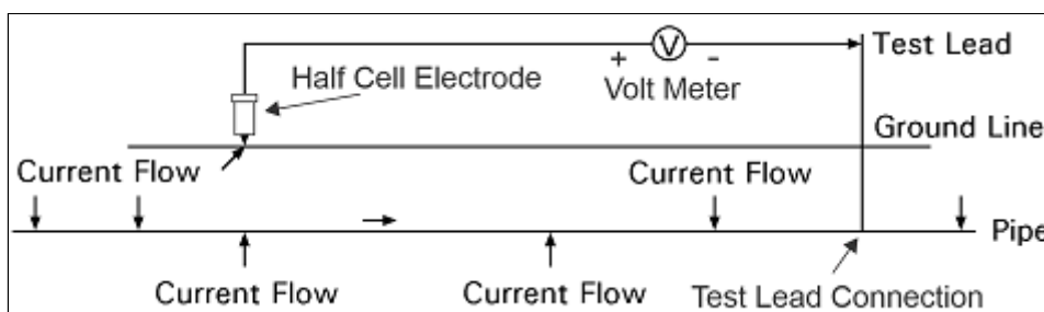
Figure 3. Cathodic Protection Current Flow Diagram
