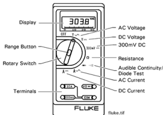
Figure 1 -Typical Multimeter
