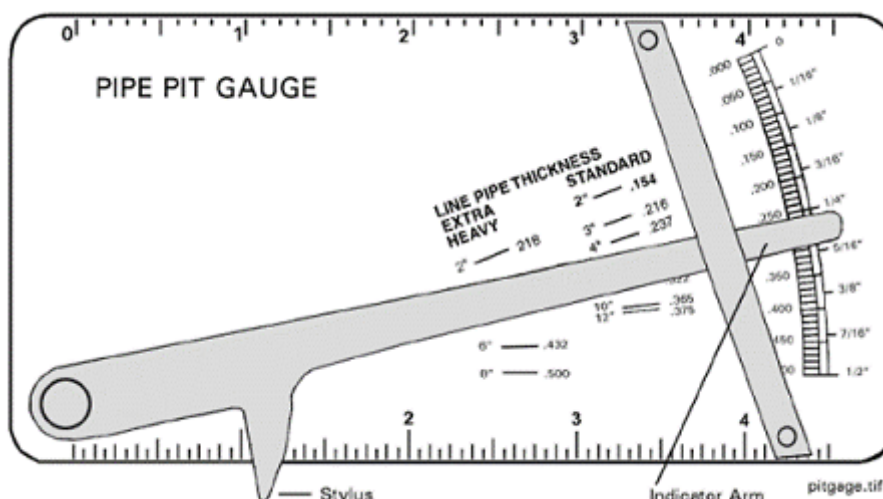
Figure 2 Pipe Pit Gauge (AG-1151, Stock Code 61 12 168)
