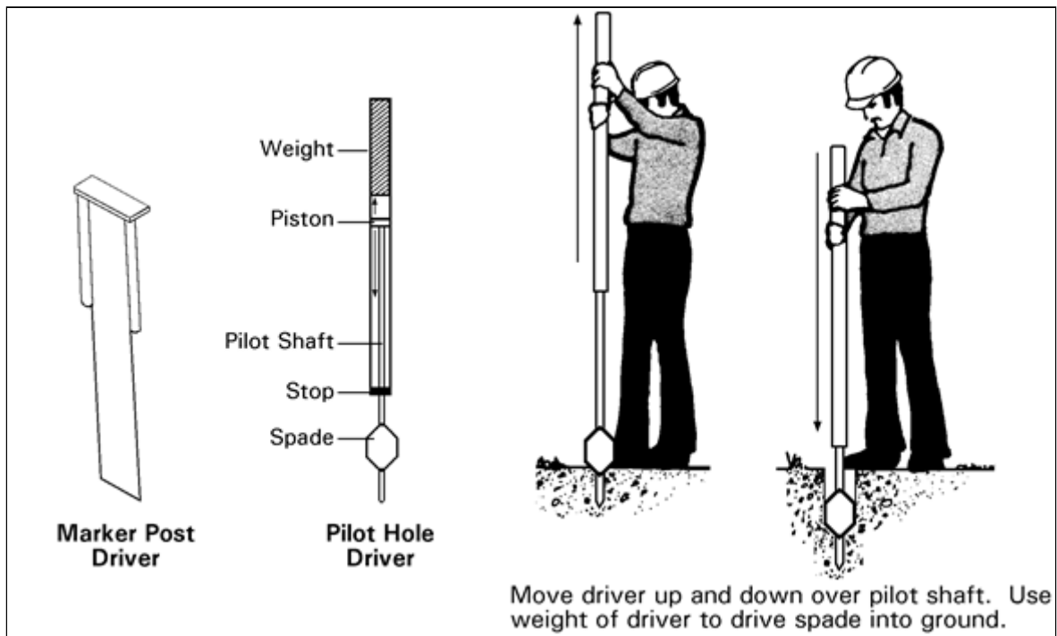
Figure 4: Pilot Hole Driver Installation
