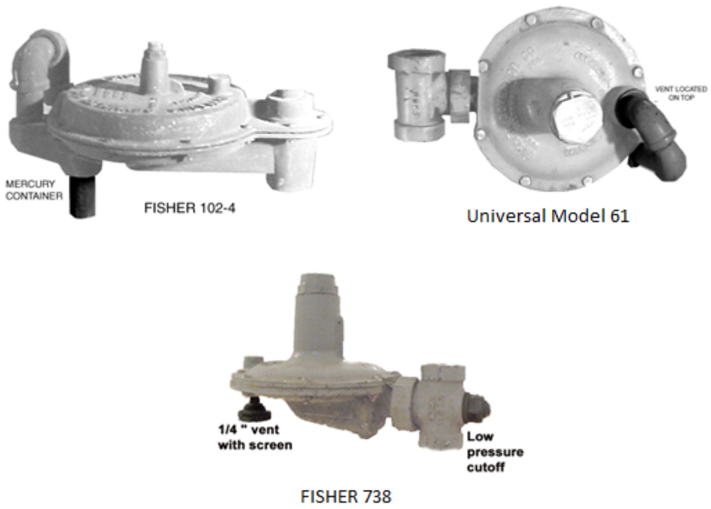
Figure B-2: Substandard Regulators
