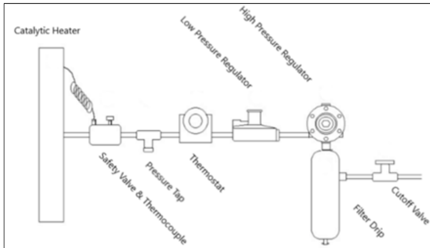
Figure 5: Catalytic Heater Control Schematic
