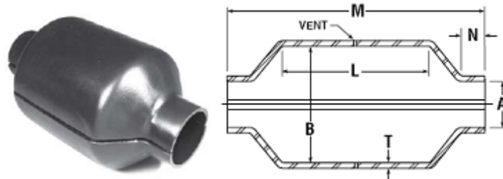
Figure 2: Dresser Style 220 Sleeve
