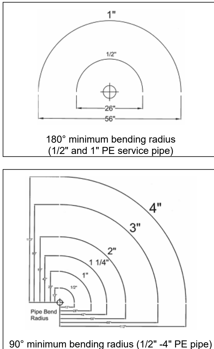
Figure 1: Permanent Minimum Pipe Bend Radius (Pipe WITHOUT Fittings)
