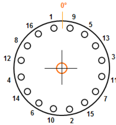
16 Bolts Sequential Order
