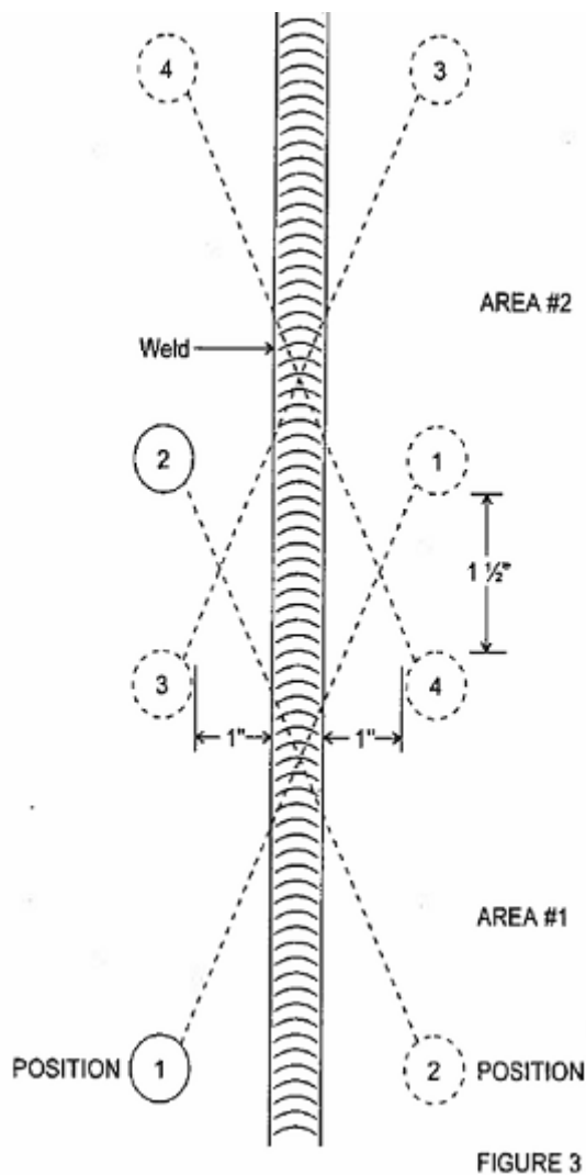
Figure 3: Magnetic Particle Inspection Sequence
