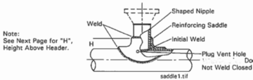
Figure 1: Regular Type Reinforcing Saddle - Typical Installation
