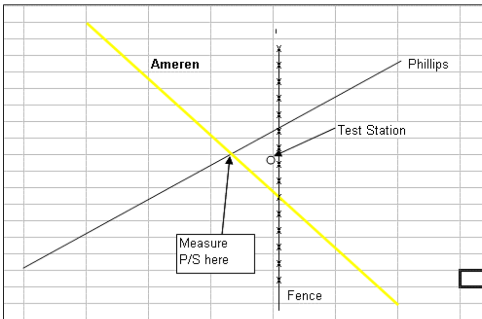
Figure 8 Foreign Pipeline Crossing Diagram
