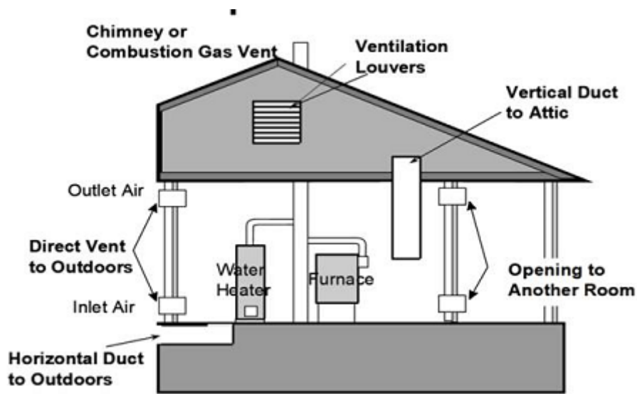
Figure 1: Air Openings for Combustion and Ventilation Air
