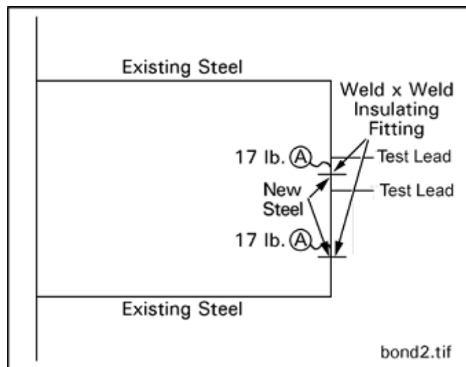
Figure 6. Steel System Loop
