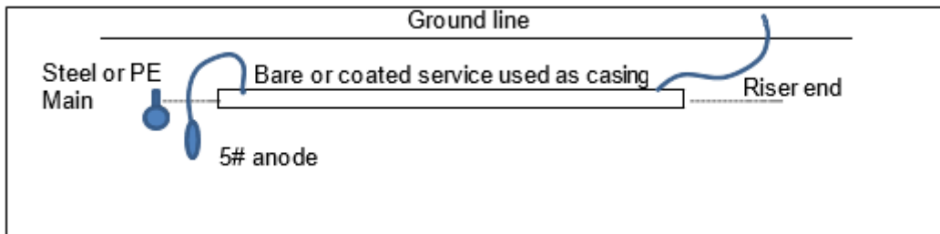
Figure 2. Anode Installation for Casing
