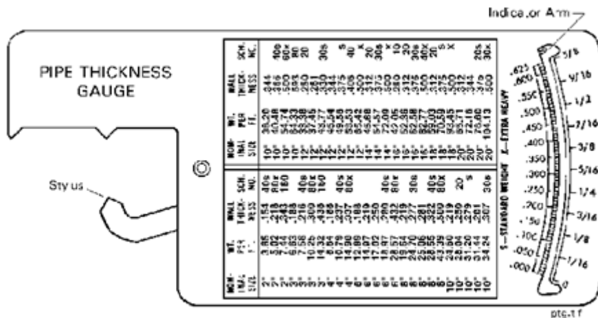
Figure 3 Pipe Thickness Gauge (AG-1153, Stock Code 85 20 170)
