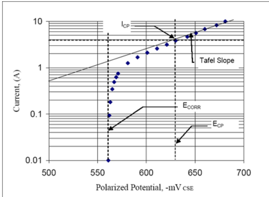
Figure 2. E-log-I Curve showing Tafel Slope
