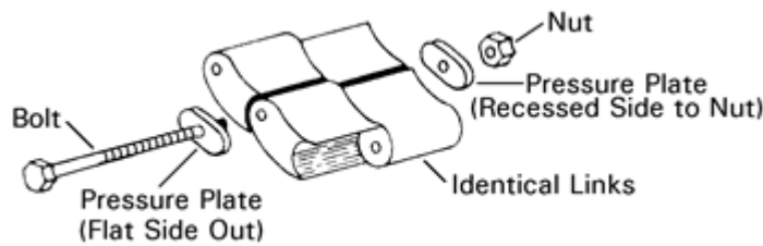
Figure 5: Link assembly
